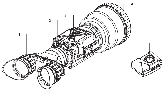
FIGURE 3-5. CONTROLS
