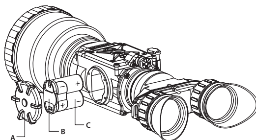
FIGURE 3-1. BATTERY INSTALLATION
