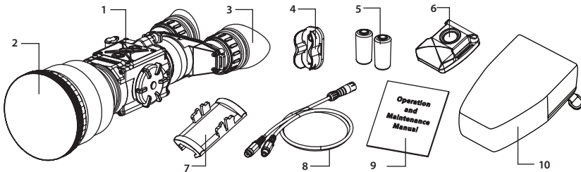
FIGURE 2-3. STANDARD COMPONENTS
