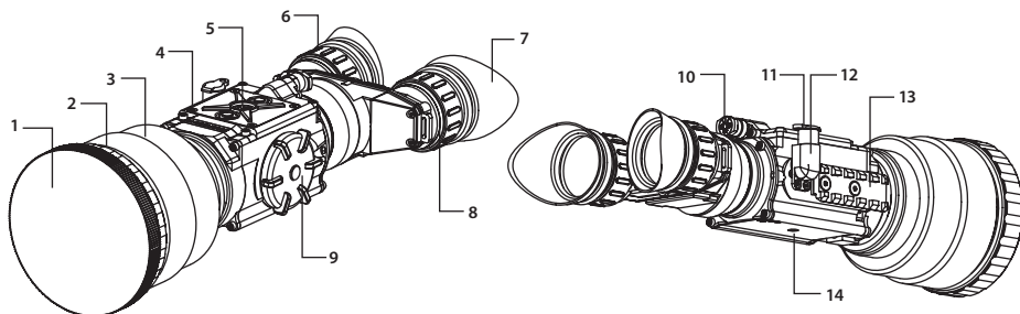
FIGURE 2-2. HELIOS HD THERMAL IMAGING BI-OCULAR. SYSTEM DESCRIPTION
